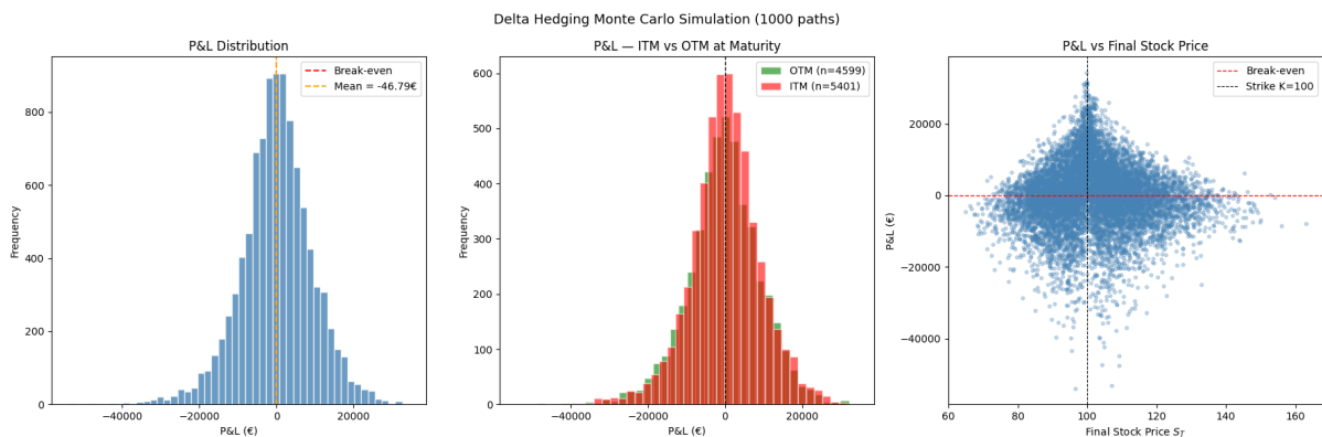
FIGURE 17 – Distribution du P&L du Delta Hedging - Simulation Monte Carlo
